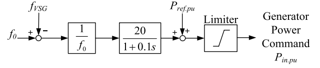
Fig. 3. Governor diagram.
