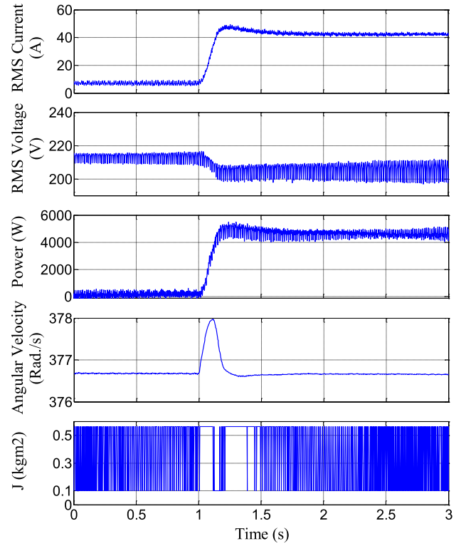
Fig. 21. RMS current, RMS voltage, output power, virtual angular velocity, and virtual moment of inertia of VSG with alternating J and D = 17 \text{ pu} after a power command of 4.5 kW.
