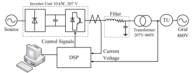
Fig. 17. Experimental system.
