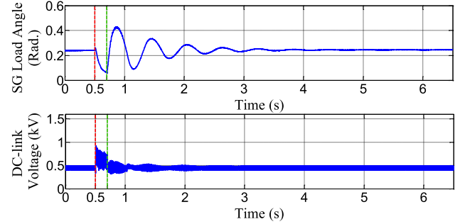
Fig. 16. SG load angle and dc-link voltage of the system of Fig. 14 containing VSG with alternating inertia.
