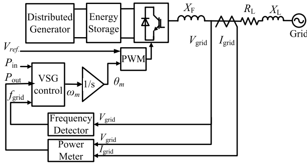
Fig. 1. Block diagram of VSG unit.
